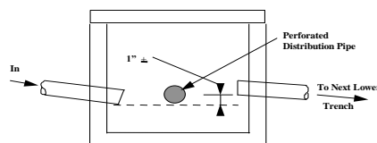
Reversed Distribution Box
