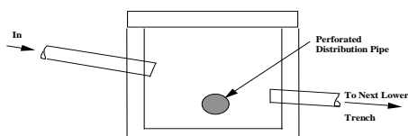
High - Level Overflow Dist. Box
